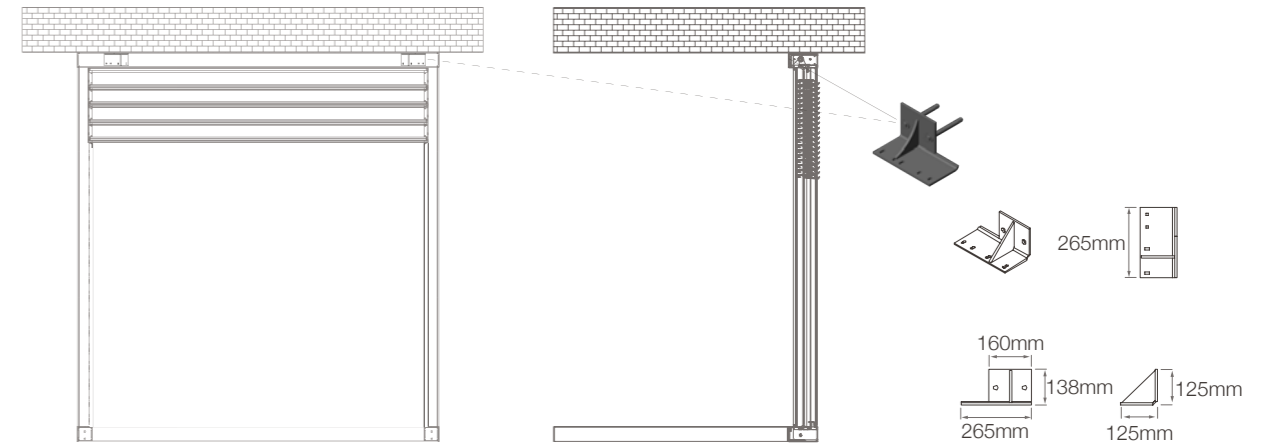
Inner (Hidden) Wall Bracket (Inox)
